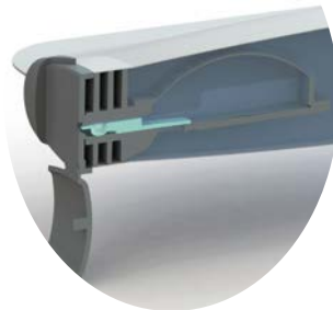
Valve Twin-Flex
